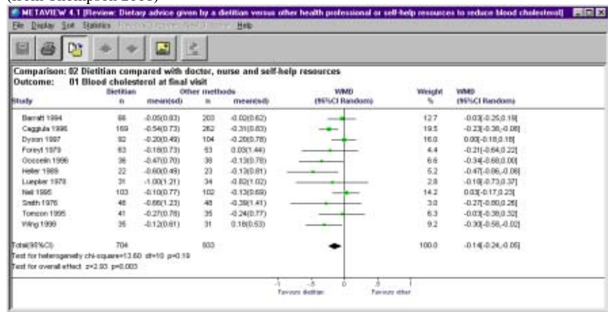
Figure 1: Forest plot from a Cochrane Review of dietary advice for cholesterol reduction (from Thompson 2001)
