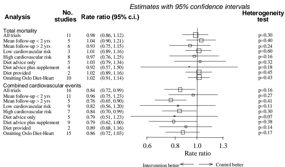
Figure 2: Forest plot of subgroup analyses and sensitivity analyses from a review of trials of reduction/modification of dietary fat or cholesterol (data from Hooper 2001)
